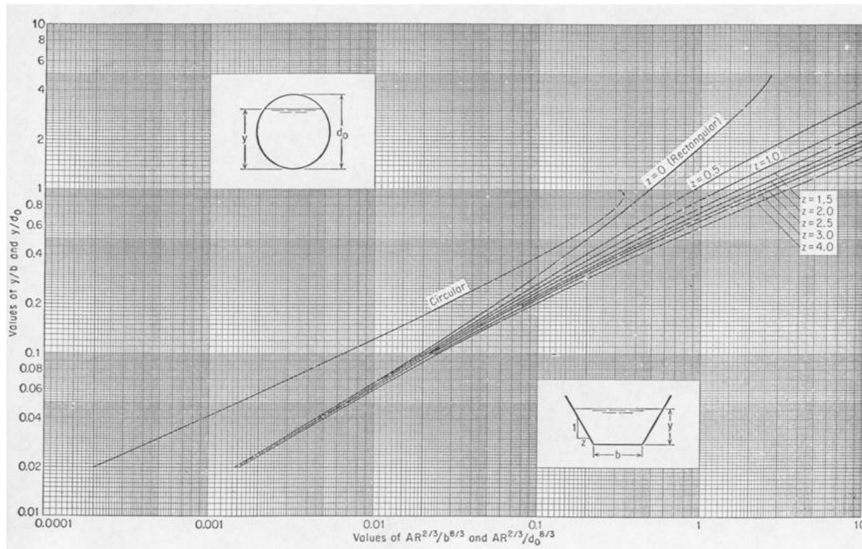
Figure 5-8. Chow (1959) curves for determining normal depth for various channel geometries.
