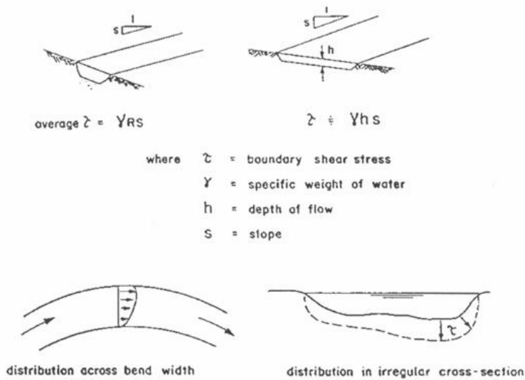
Figure 5-3. Boundary shear stress in uniform flow (COE 1994).
