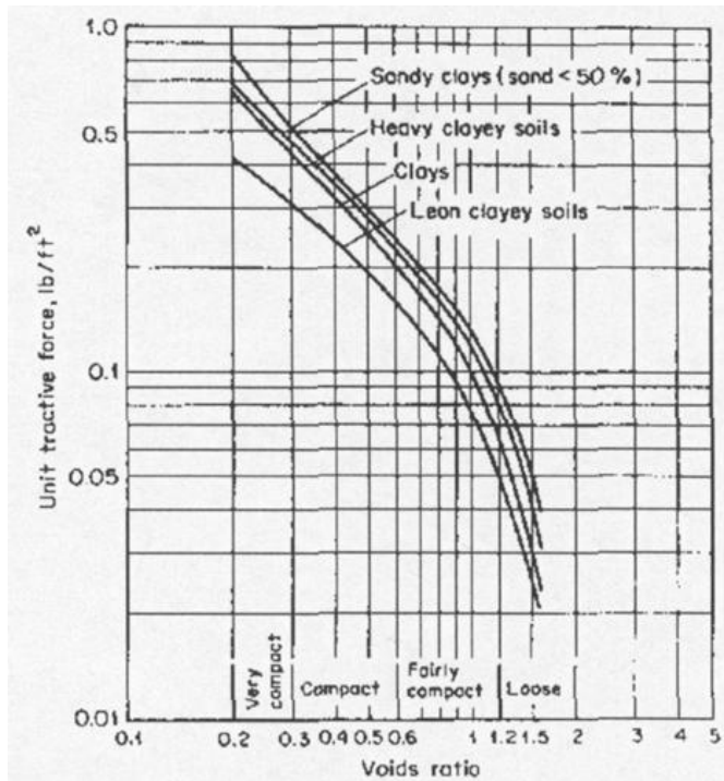
Figure 5-6. Example of allowable shear stresses (tractive forces) for cohesive materials (COE 1994).
