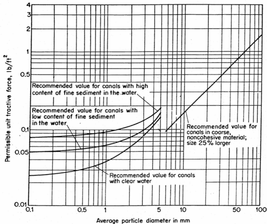
Figure 5-5. Allowable shear stresses (tractive forces) for canals in granular materials (U.S. Bureau of Reclamation, reprinted in Chow 1959).
