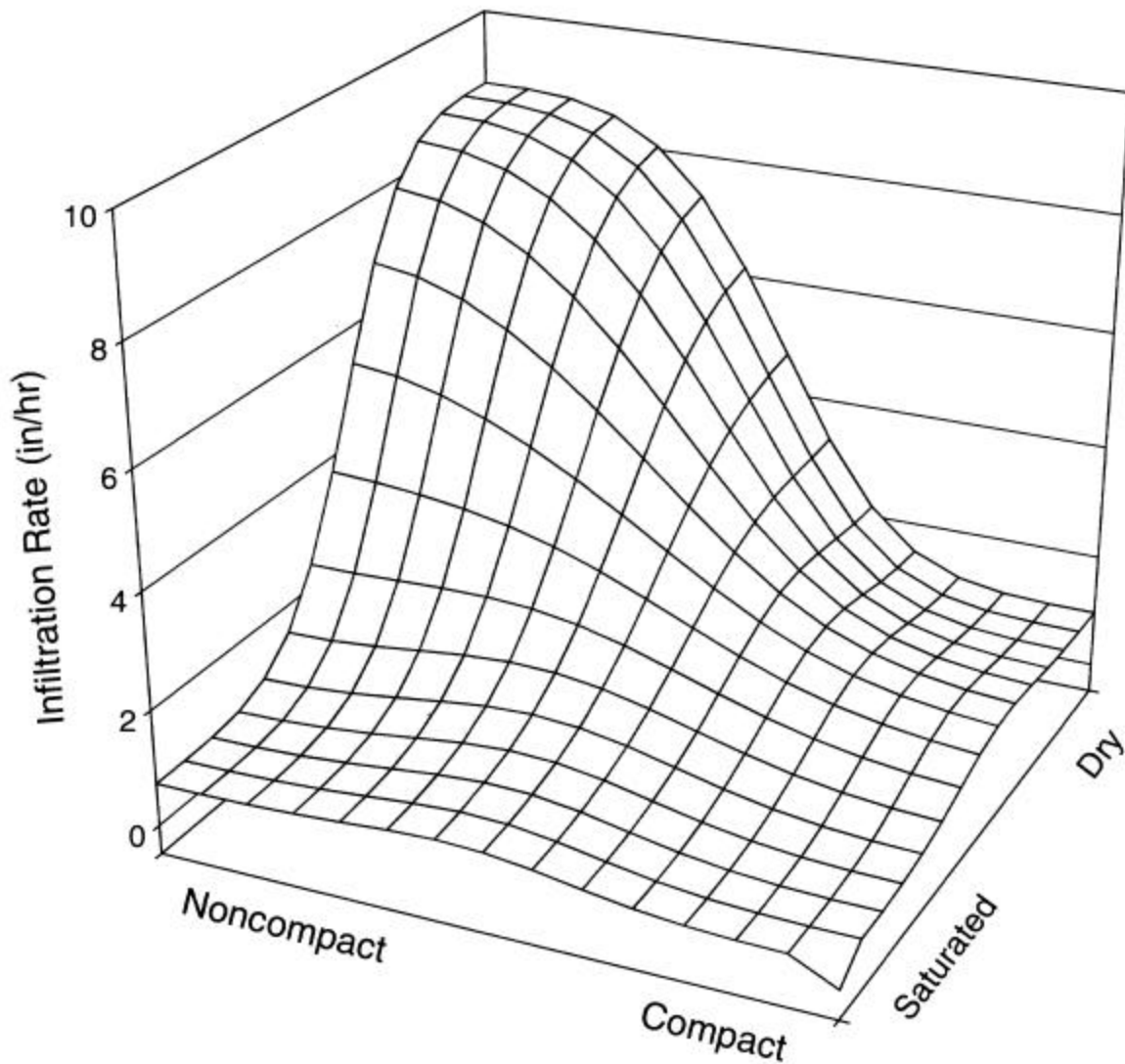
Figure 3-2. Three dimensional plot of infiltration rates for clayey soil conditions.
