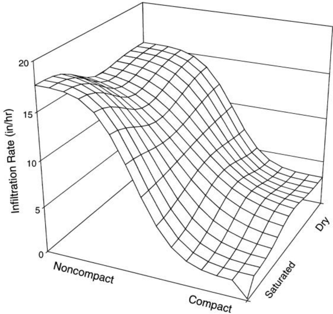
Figure 3-1. Three dimensional plot of infiltration rates for sandy soil conditions.
