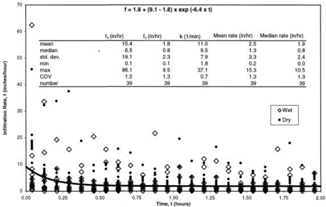
Figure 3-4. Infiltration measurements for compacted, sandy soil, conditions.
