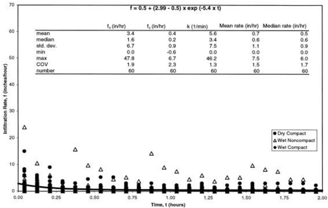
Figure 3-6. Infiltration measurements for wet-noncompacted, dry-compacted, and wet-compacted, clayey soil conditions.
