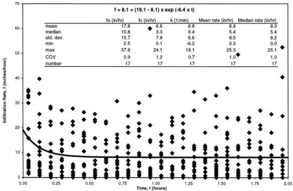
Figure 3-5. Infiltration measurements for dry-noncompacted, clayey soil, conditions.
