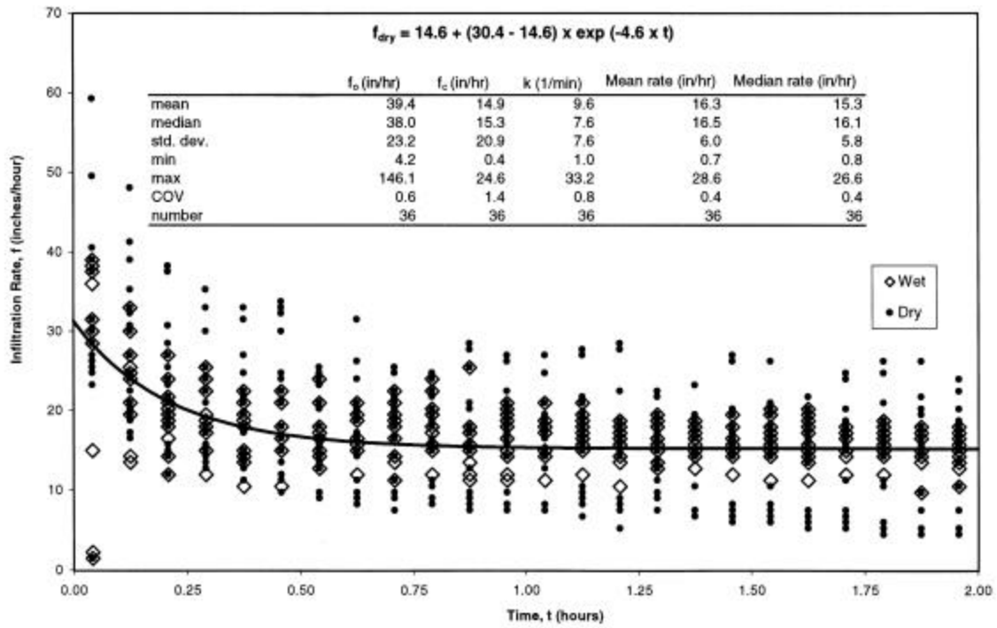
Figure 3-3. Infiltration measurements for noncompacted, sandy soil, conditions.
