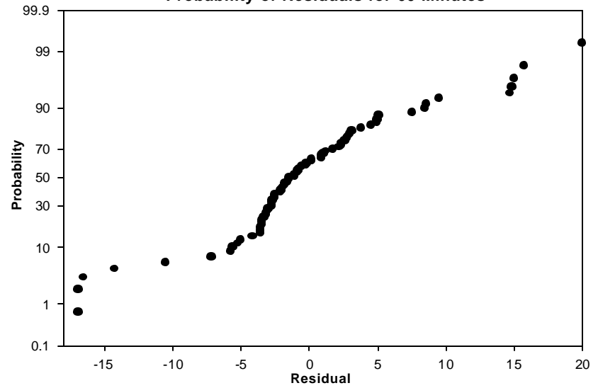
Probability of Residuals for 60 Minutes
