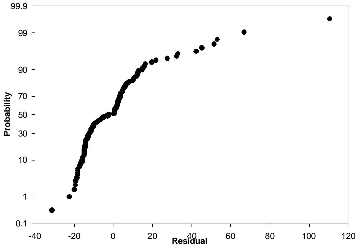
Figure 3-20. Probability plot of the residuals resulting from the comparison of the model to the observed values.
