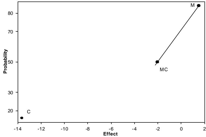
Probability of Effects for 60 Minutes
