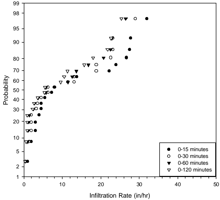
Figure 3-9. Probability plots for infiltration measurements for dry-noncompacted, clayey soil, conditions.
