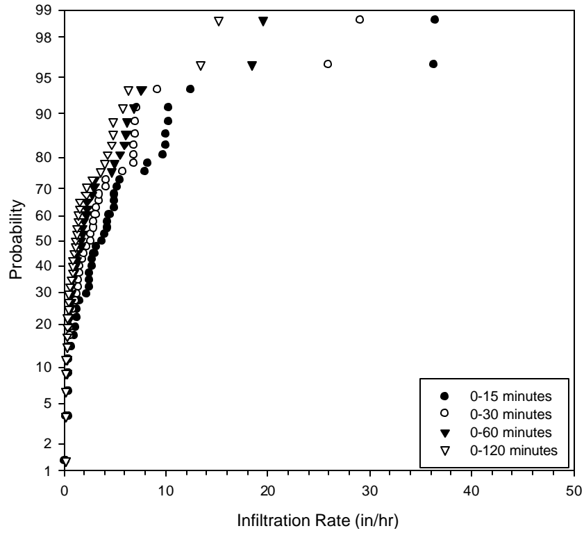
Figure 3-8. Probability plots for infiltration measurements for compacted, sandy soil, conditions.
