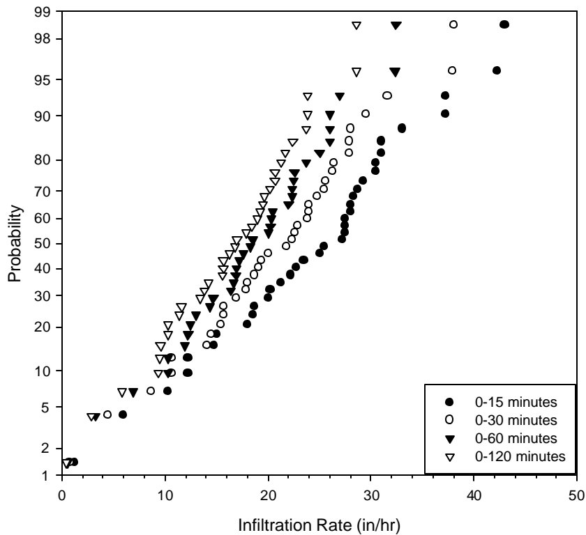
Figure 3-7. Probability plots for infiltration measurements for noncompacted, sandy soil, conditions.
