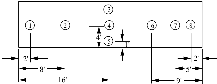
Detail of Soil Sampling Scheme
