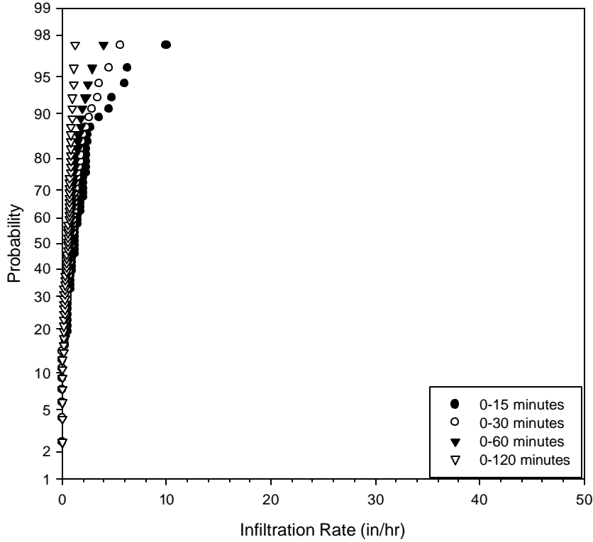
Figure 3-10. Probability plots for infiltration measurements for wet-noncompacted, dry-compacted, and wet-compacted, clayey soil conditions.
