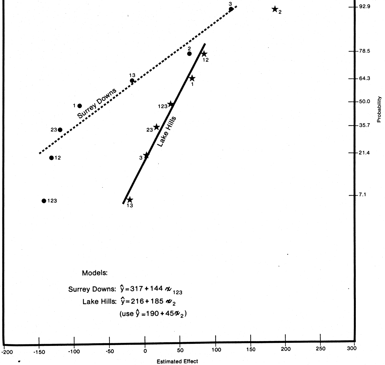
2 3 Factorial Analysis Results for Experimental Design Street Particulate Loading Data
