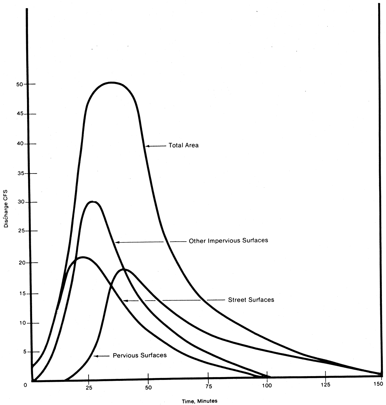
FIGURE 5-9 Hypothetical Hydrograph for Urban Watersheds
