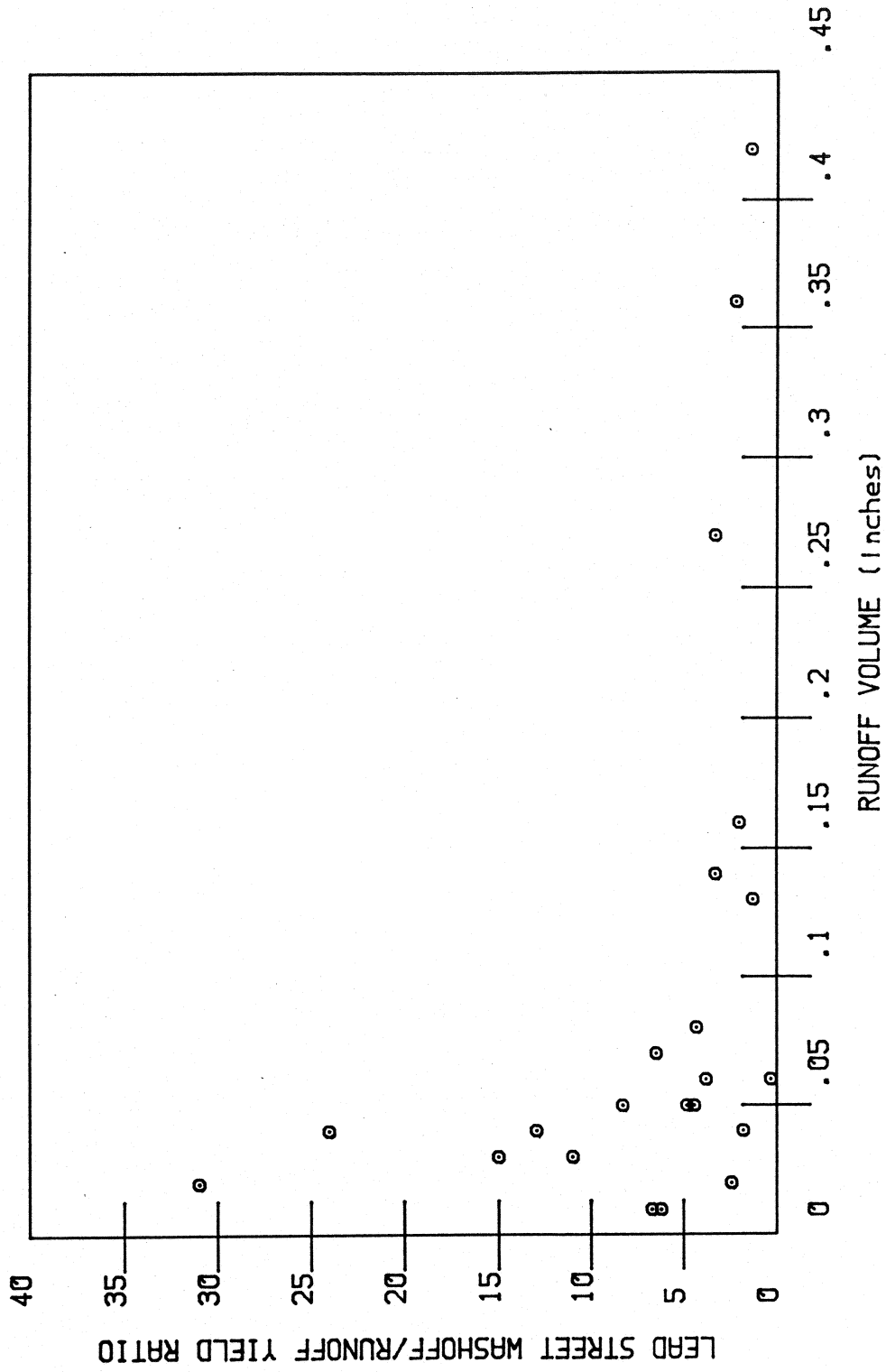
FIGURE 9-19 LEAD WASHOFF/RUNOFF YIELD
