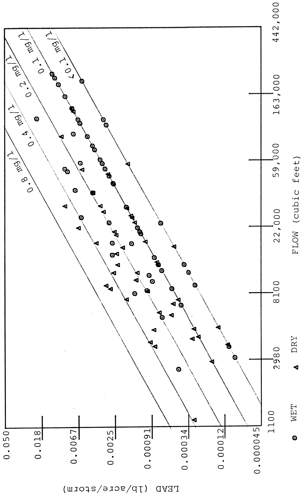
FIGURE 6-7 LAKE HILLS - Lead by Season
