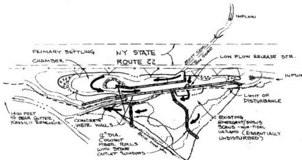
Figure 71. Bear Gutter Creek highway right-of-way urban stormwater retrofit (Claytor 1998).
