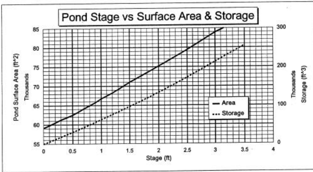
Figure 35. Pond-stage surface area relationship for example problem.
