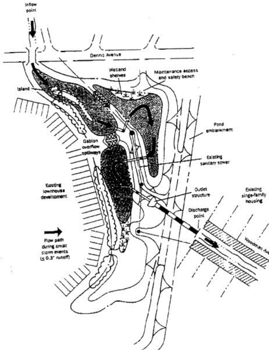
Figure 70. Wheaton Branch, Maryland, detention facility retrofit project (Claytor 1998).
