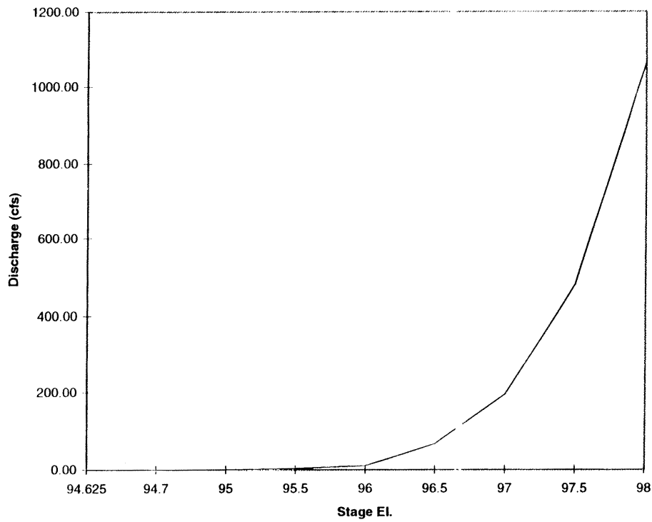
Figure 51. Stage-discharge curve for Monroe St. pond.
