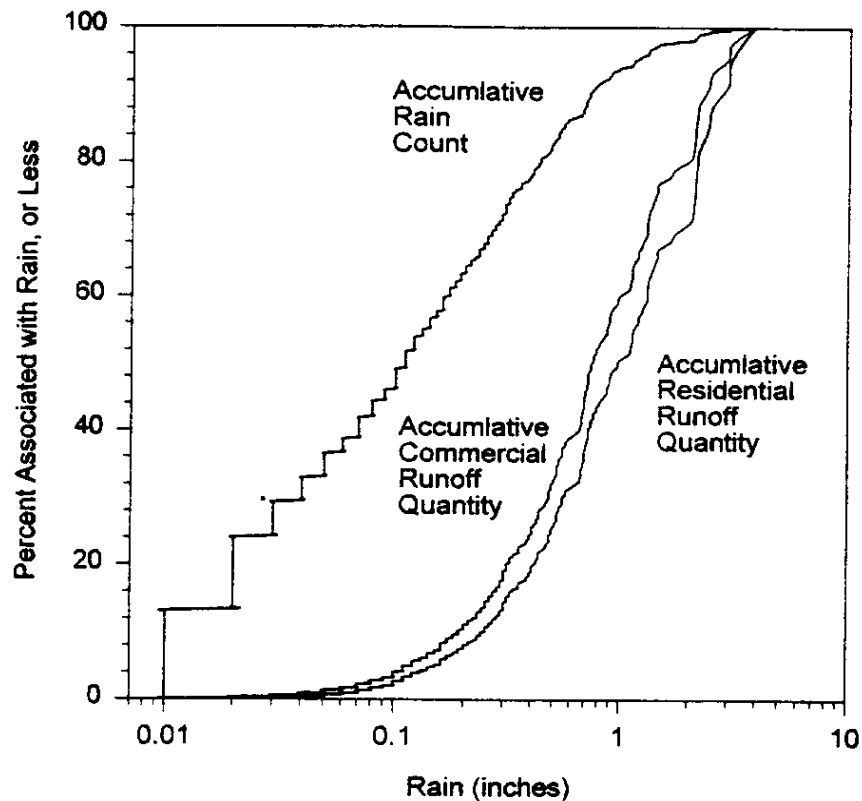
Figure 62. Recorded rain count and modeled runoff volume distributions for Minneapolis, MN (1983 through 1989).
