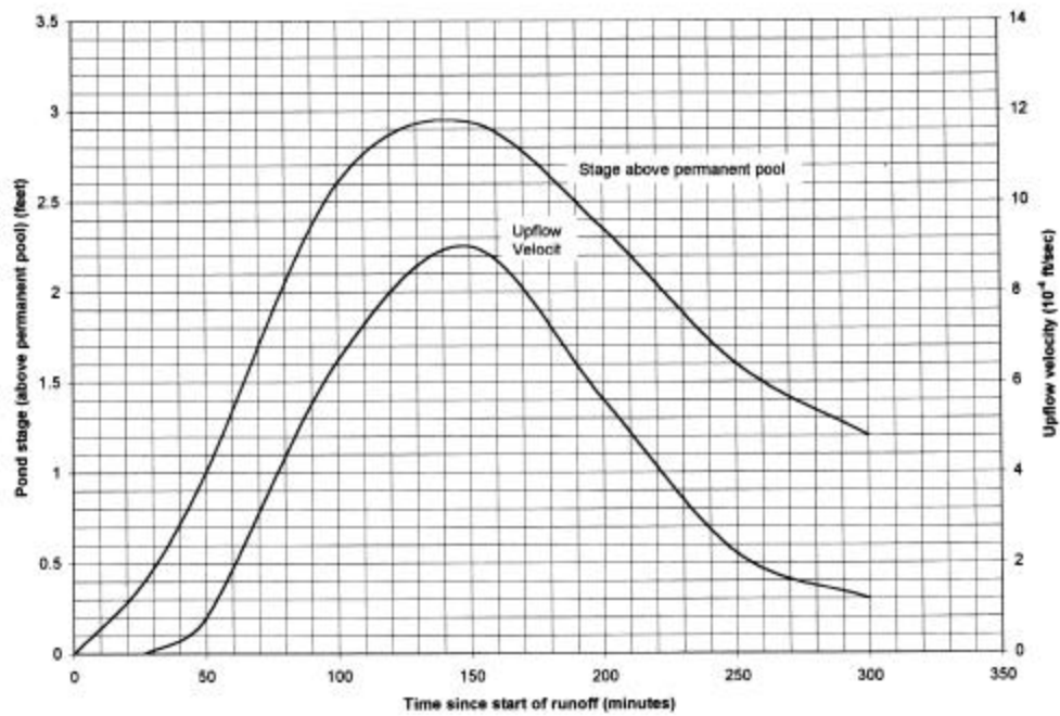
Figure 38. Stage and upflow velocity plots for example problem.
