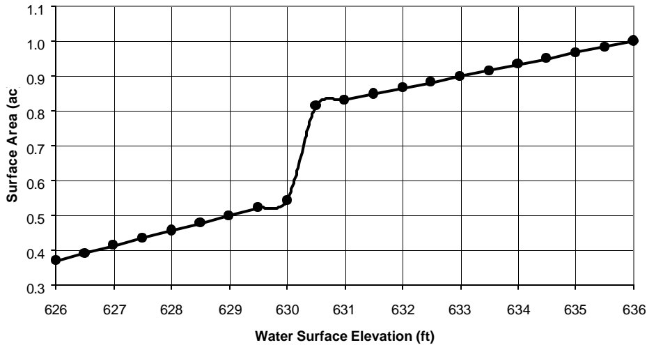
Figure 58. Stage v. Surface Area Curve
