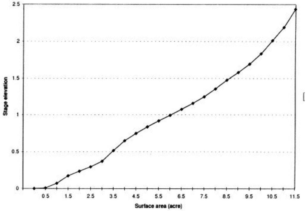
Figure 50. Pond-surface area curve for Monroe St. pond.
