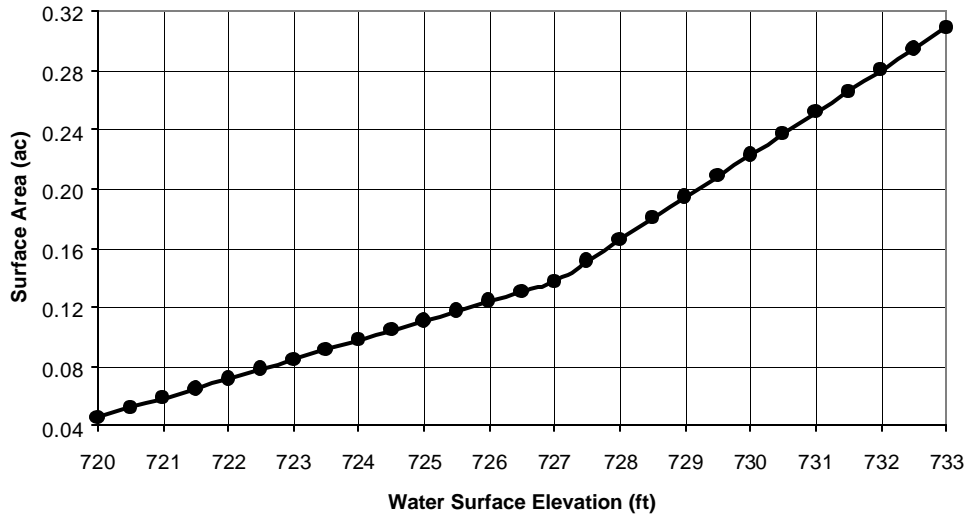
Figure 65. Stage v. Surface Area Curve.
