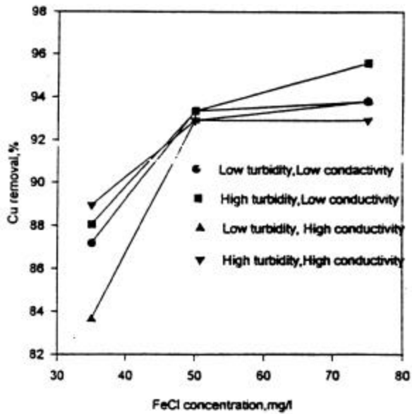
Figure 2. Copper removal using ferric chloride.
