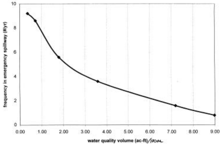
Figure 41e. Austin, TX, commercial area sensitivity analysis indicating number of spillway events per year.
