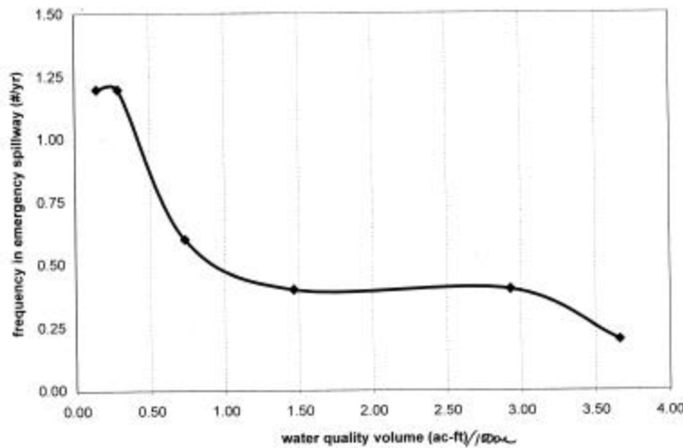
Figure 41h. Minneapolis, MN, medium density residential area sensitivity analysis indicating number of spillway events per year.
