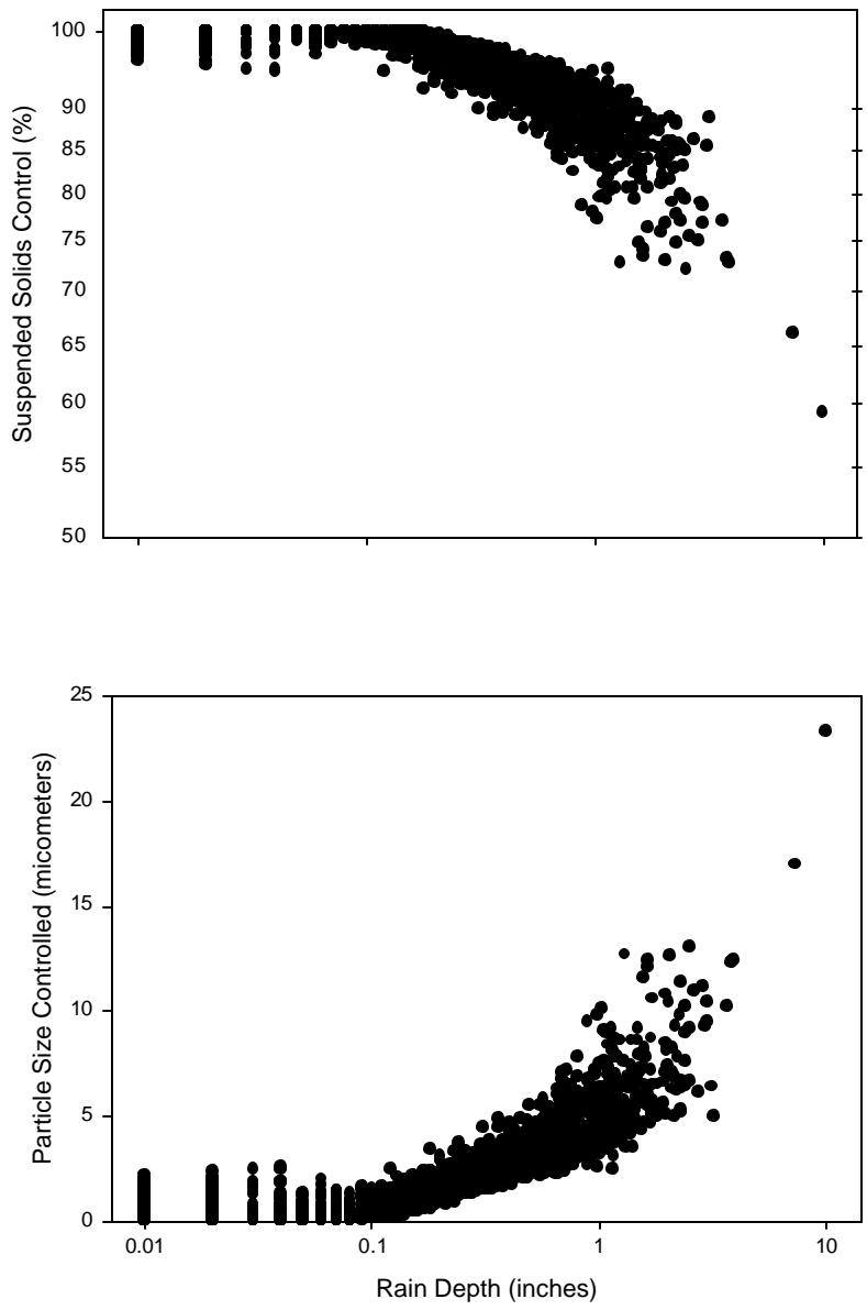
Figure 63. Suspended solids and particulate control as a function of rain depth.
