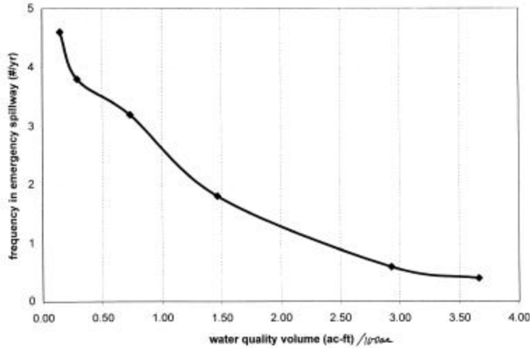
Figure 41g. Austin, TX, medium density residential area sensitivity analysis indicating number of spillway events per year.
