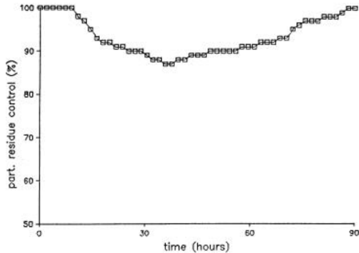
Figure 43. Modeled detention pond suspended solids removal performance for 4.1 inch, 24-hour rain example.
