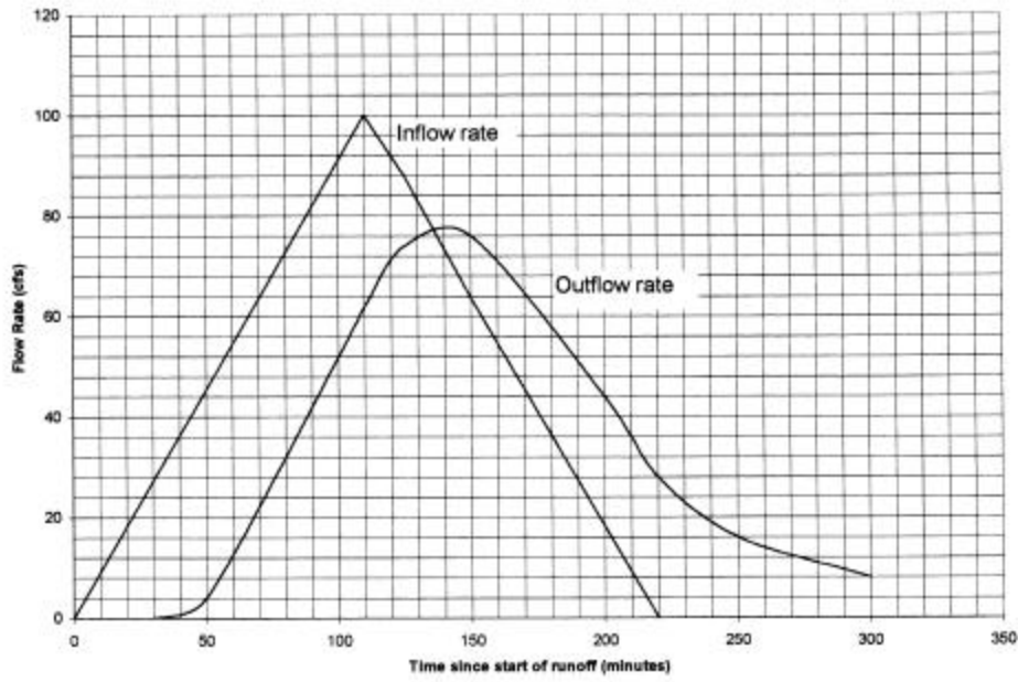
Figure 37. Inflow and outflow hydrographs for example problem.
