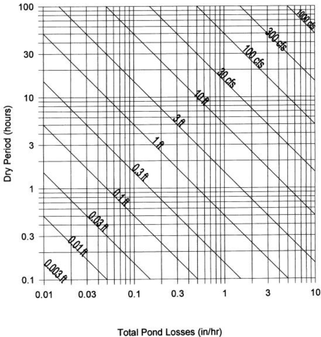
Figure 27. Pond water surface elevation drop (ft.) if no pond inflow during dry periods.
