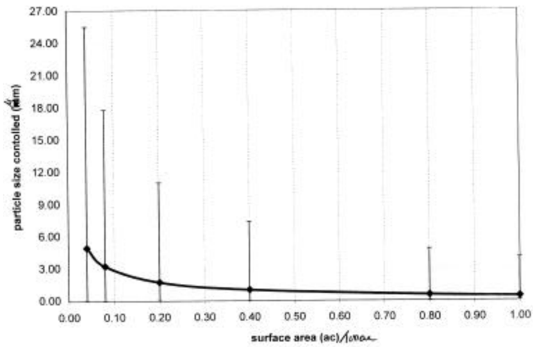
Figure 41d. Minneapolis, MN, medium density residential area sensitivity analysis based on surface area of pond.
