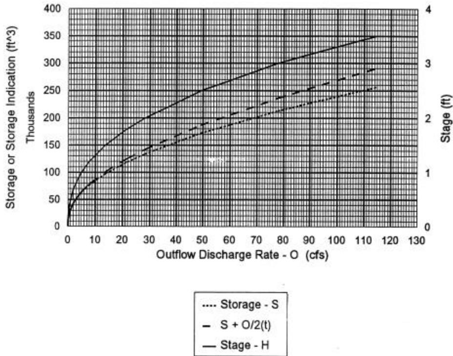
Figure 36. Pond-stage/storage indication curve for example problem.
