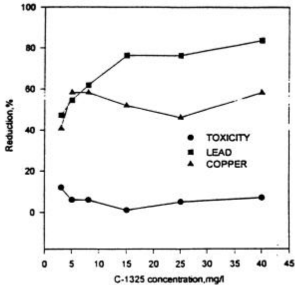
Figure 5. Metals and toxicant reductions using organic polymer (C-1325).
