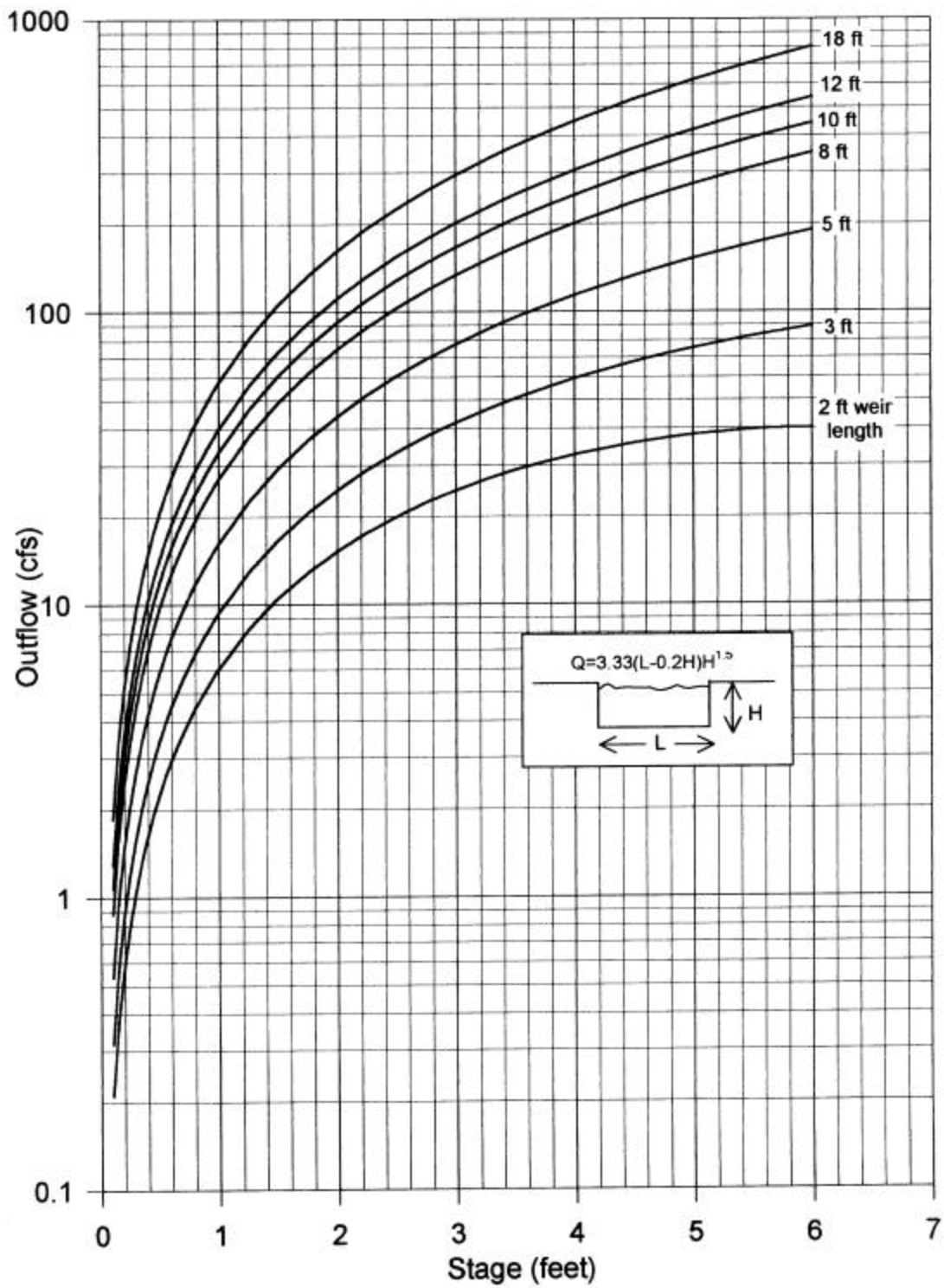
Figure 32. Approximate rating curves for rectangular weirs.
