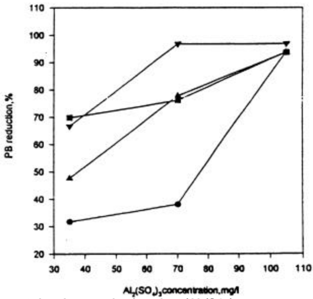
Figure 3. Lead removal using alum (Al 2 (SO 4 ) 3 )
