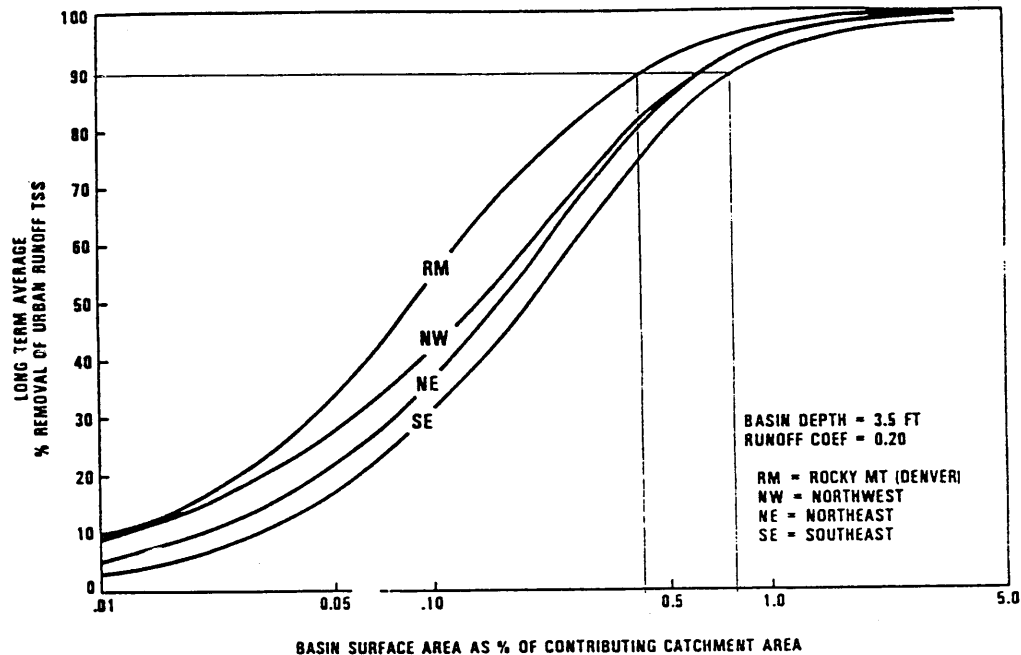
Figure 31. Regional differences in detention pond performance (EPA 1983).
