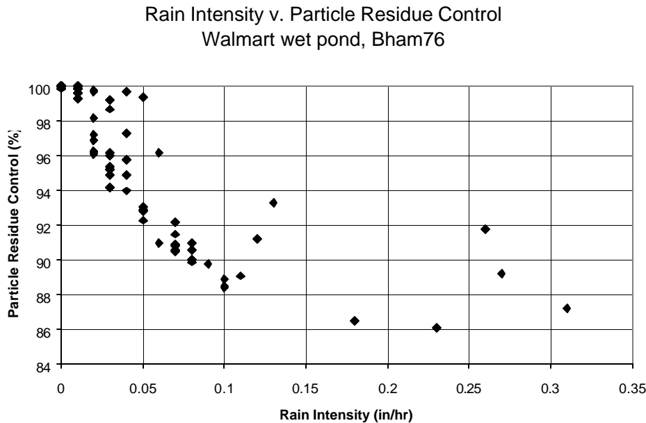
Figure 61. Rain Intensity v. Particle Residue Control
