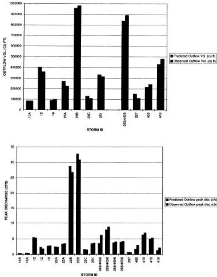
Figure 52. Predicted and observed flow volumes and peak flow rates.
