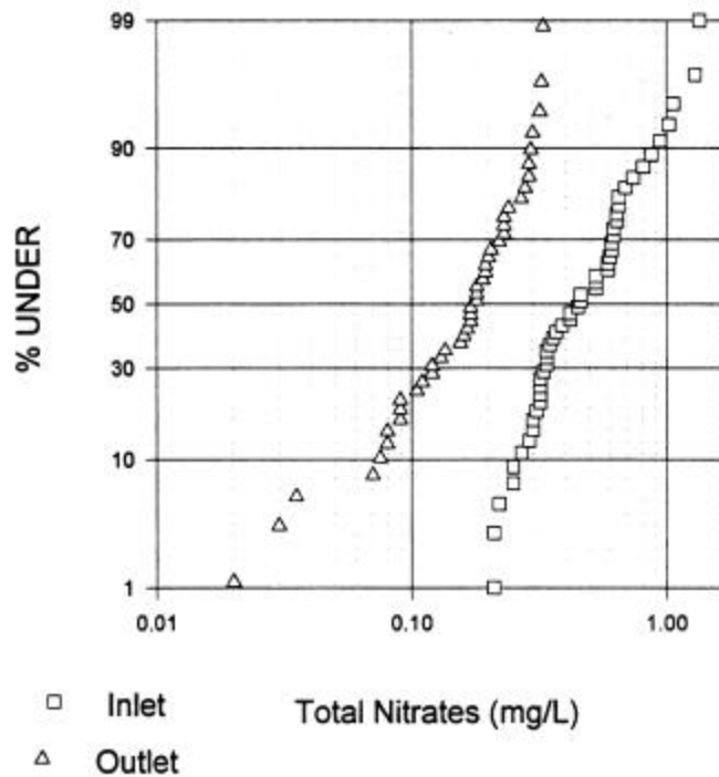
Figure 54. Probability plots of influent and effluent pollutant concentrations.
