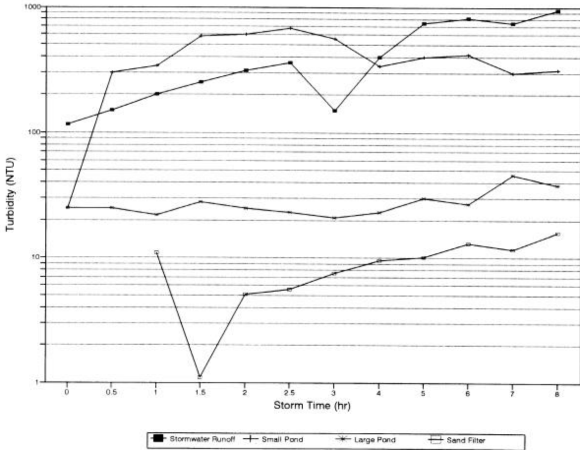
Figure 56e. Turbidity changes with time for influent, initial small pond, pond, and sand filter effluent for storm #1.
