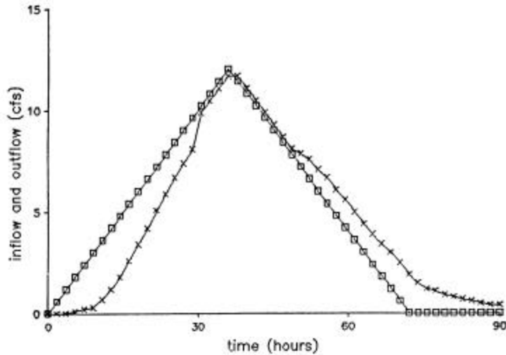
Figure 42. Modeled detention pond outflow hydrograph for 4.1 inch, 24-hour rain example.
