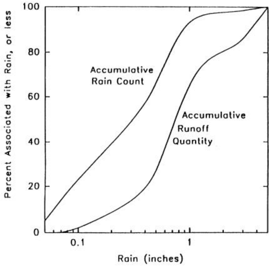
Figure 57. Milwaukee rain and runoff cumulative probability density functions (CDFs).
