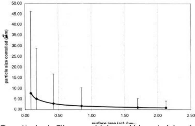
Figure 41a. Austin, TX, commercial site sensitivity analysis based on surface area of pond.
