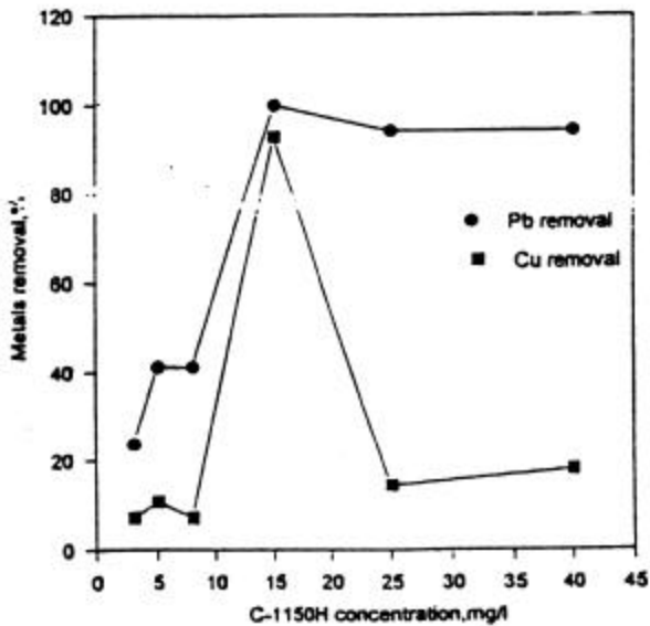
Figure 6. Metals removed using organic polymer (C-1150H).
