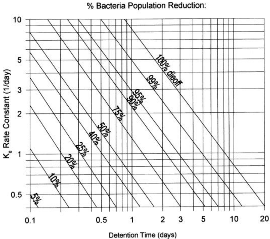
Figure 30. Chick's law for bacterial dieoff.
