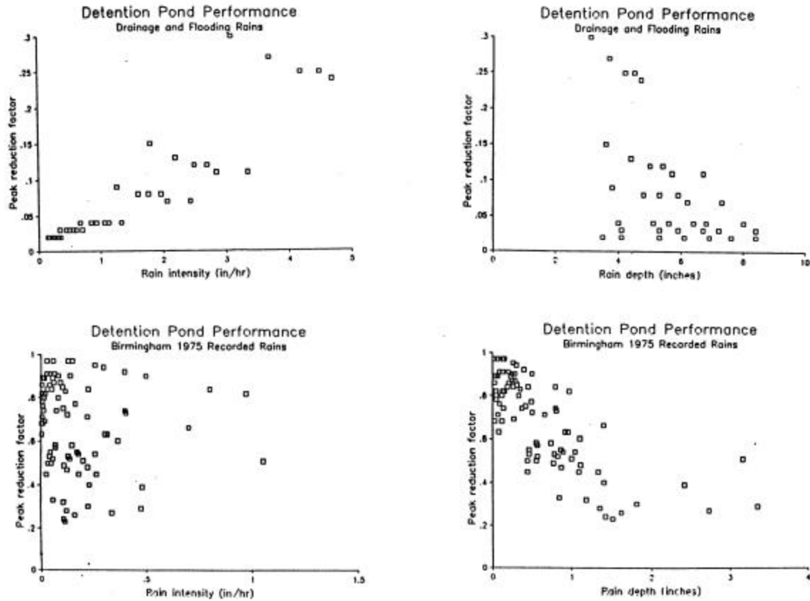
Figure 45. DETPOND modeled peak reduction factors by standard pond for various rain depths and intensities.
