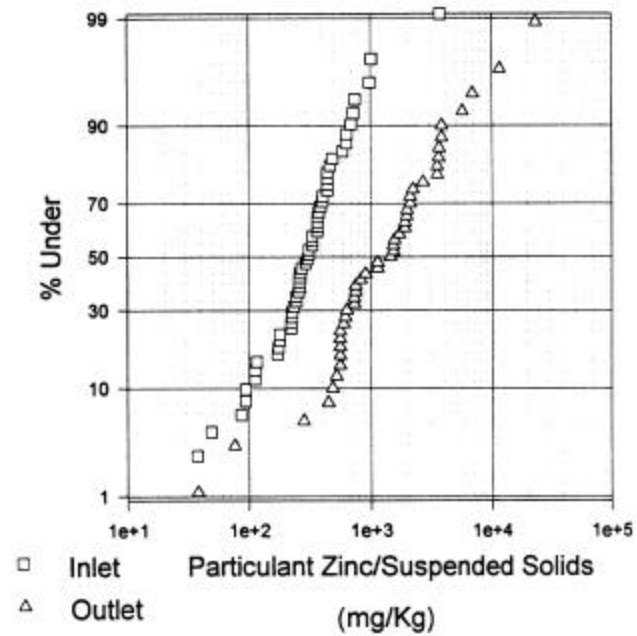
Figure 55. Particulate pollutant strengths.
