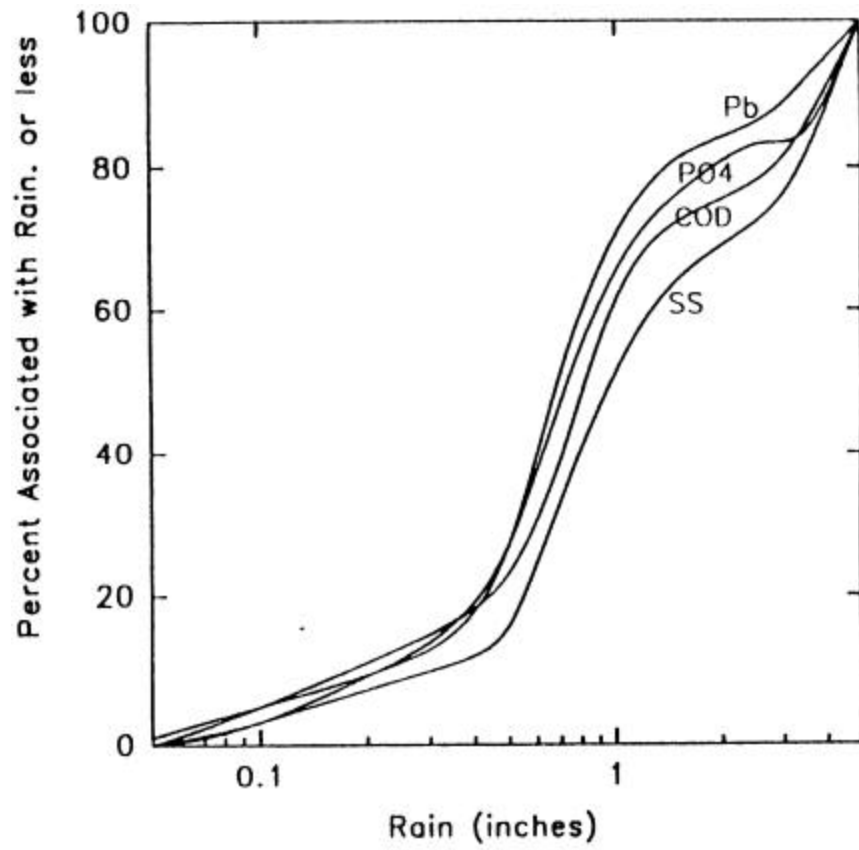
Figure 58. Milwaukee pollutant discharge cumulative probability density functions (CDFs).
