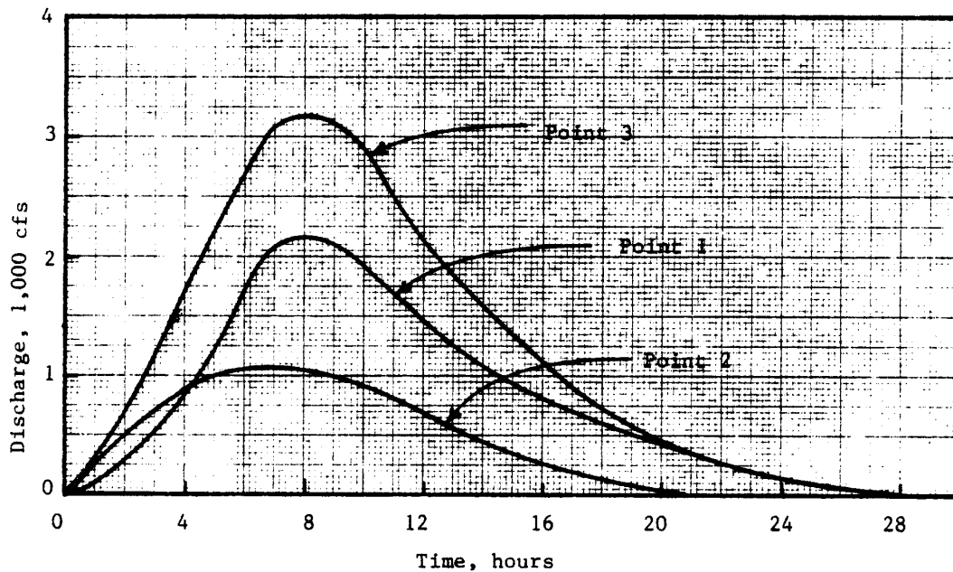
Figure 14. Hydrographs after urbanization with downstream detention (Rosmiller 1987).
