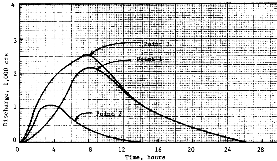
Figure 13. Hydrographs before urbanization without detention (Rosmiller 1987).
