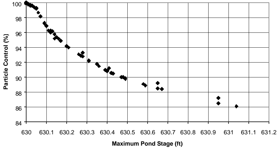
Figure 59. Pond Stage v. Particle Residue Control
