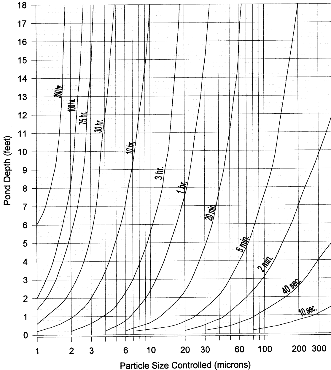
Figure 20. Required residence time for complete settling (hours).
