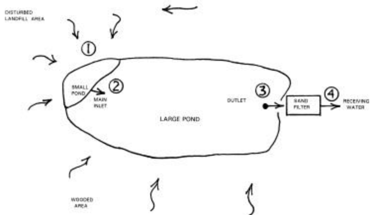
Figure 56b. Birmingham landfill and pond watershed map.
