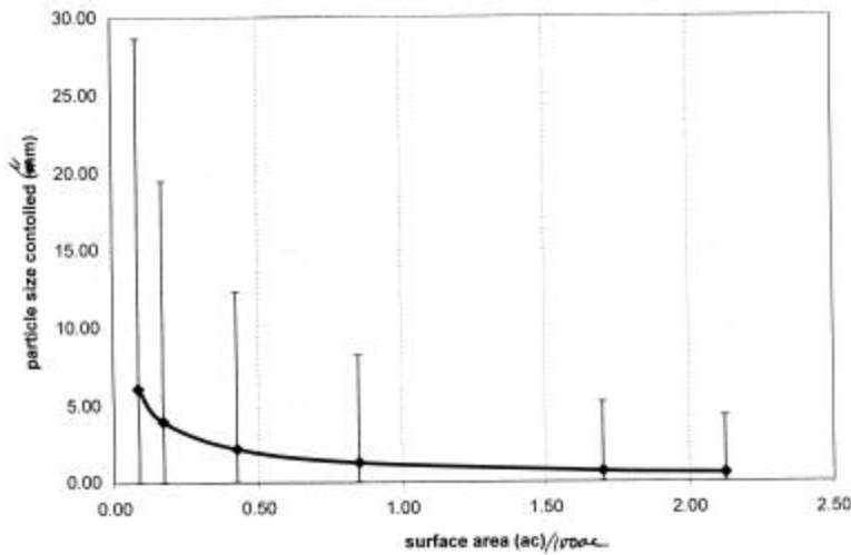
Figure 41b. Minneapolis, MN, commercial area sensitivity analysis based on surface area of pond.
