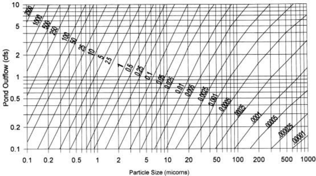
Figure 26. Minimum pond size (acres) needed for complete settling of specific sized particles at various pond overflow rates.
