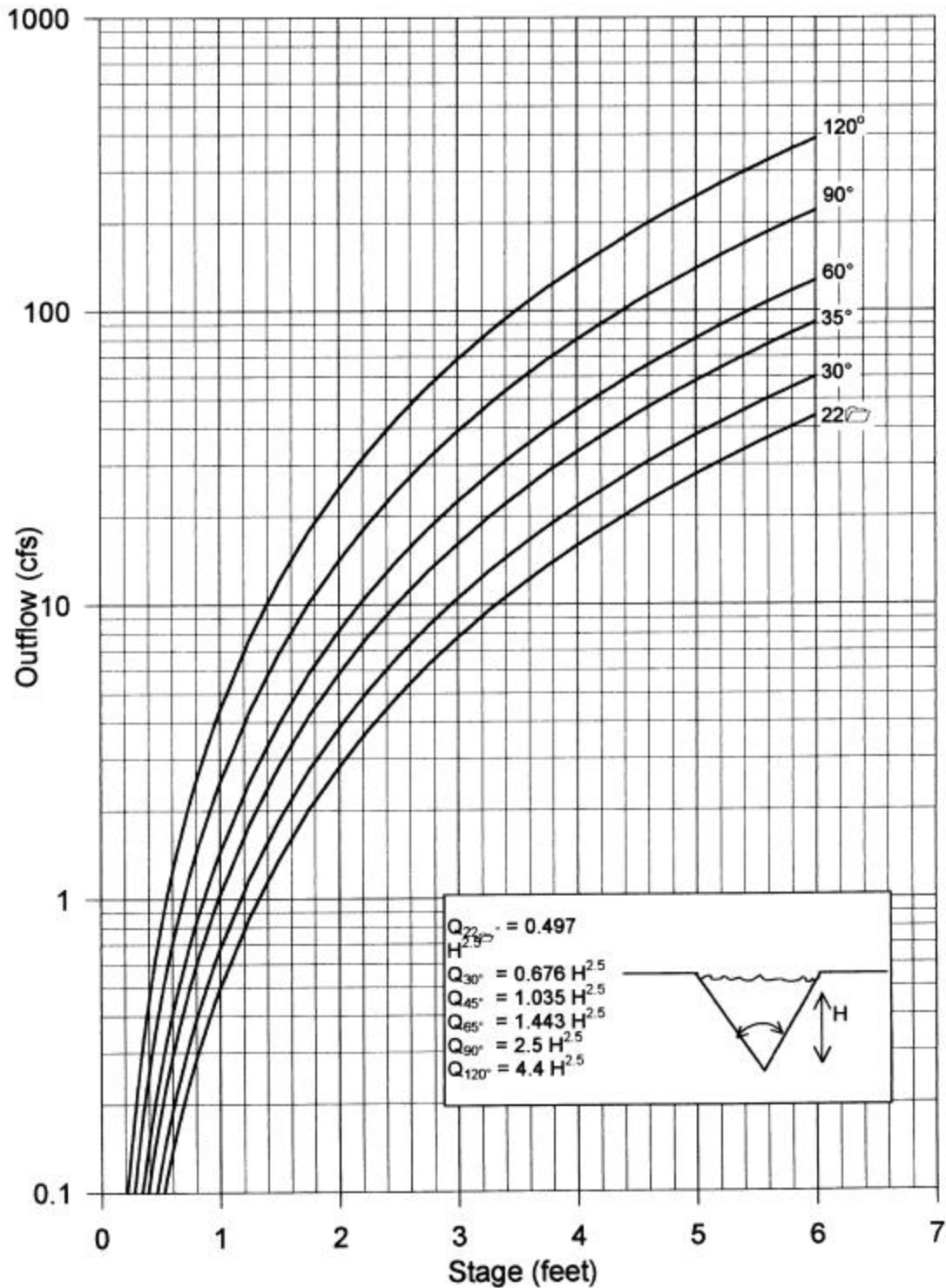
Figure 33. Approximate rating curves for V-notch weirs.
