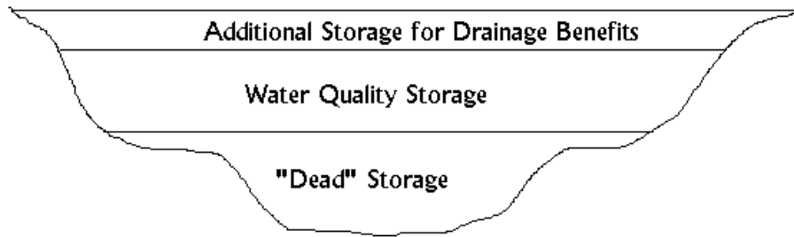
Figure 40. Cross-section of pond showing water quality storage portion
