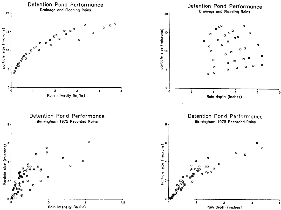
Figure 44. DETPOND modeled particle size removals by standard pond for various rain depths and intensities.
