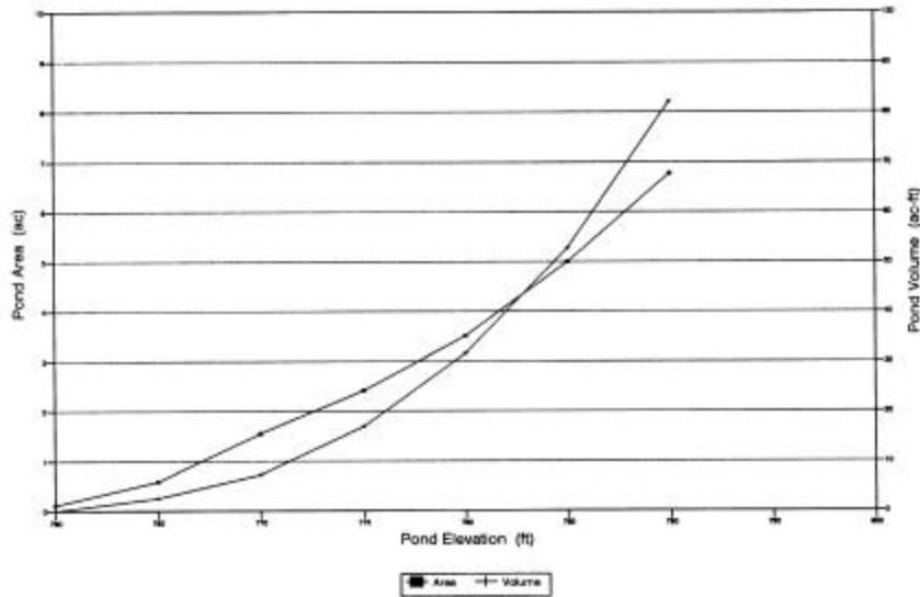
Figure 56d. Birmingham landfill elevation-area and elevation-volumes curves.
