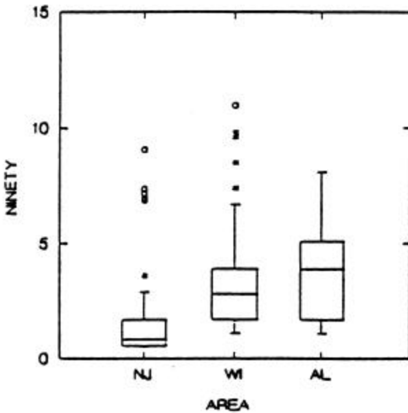
Figure 24. Ninetieth percentile particle sizes for stormwater inlet flows (Pitt, et al. 1997).
