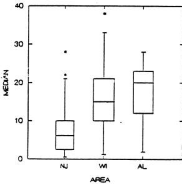
Figure 23. Fiftieth percentile particle sizes for stormwater inlet flows (Pitt, et al. 1997).
