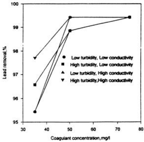
Figure 1. Lead removal using ferric chloride.
