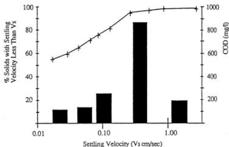
Figure 29. COD and particulate settling velocity (Butler, et al. 1993).
