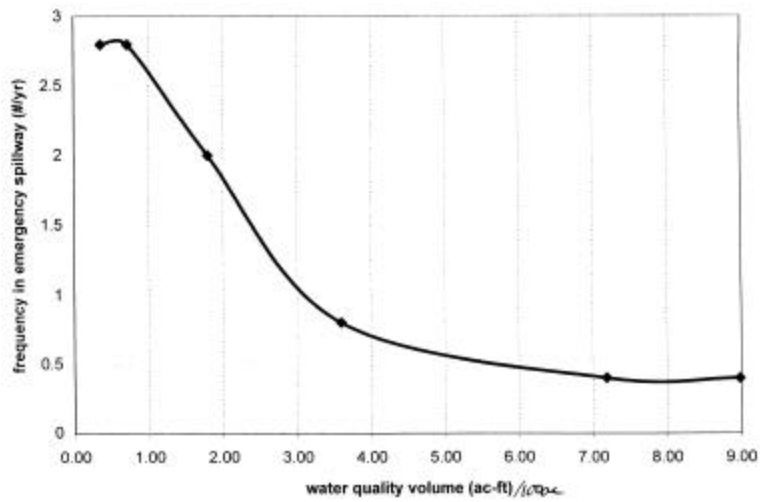
Figure 41f. Minneapolis, MN, commercial area sensitivity analysis indicating number of spillway events per year.
