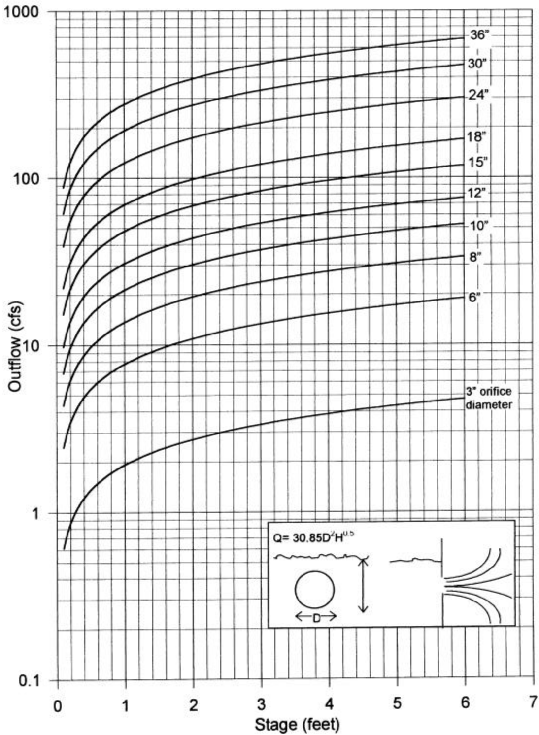
Figure 34. Approximate rating curves for orifice discharges.
