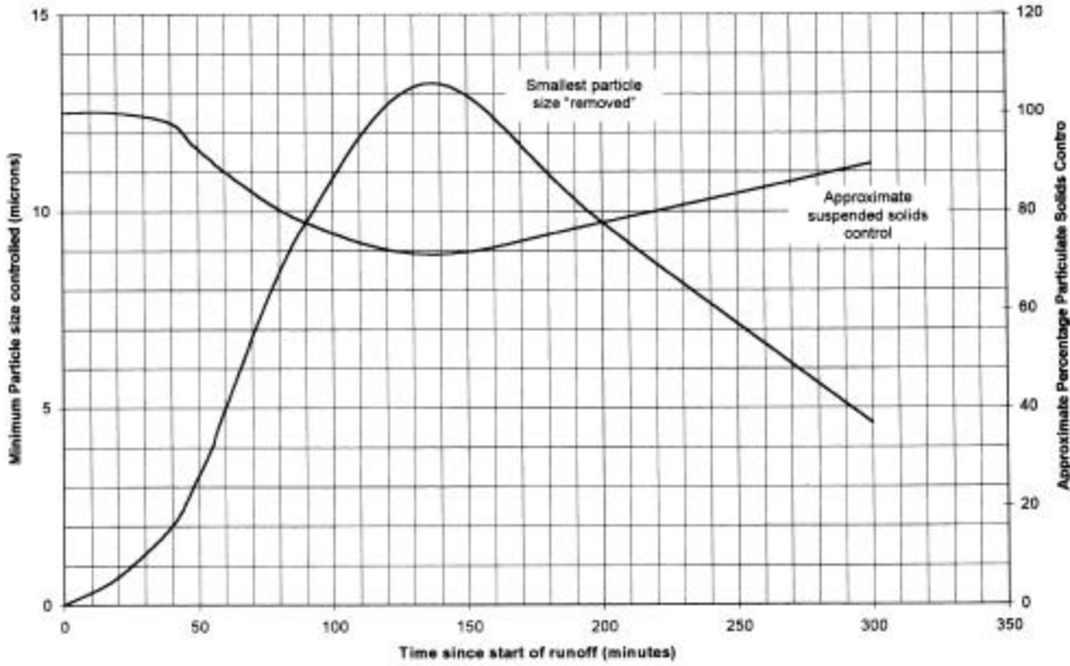
Figure 39. Particle sizes and percentage suspended solids removed for example problem.
