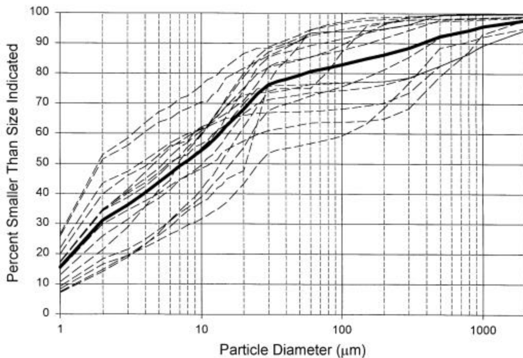
Figure 56. Inlet particle size distributions observed at the Monroe St. wet detention pond.
