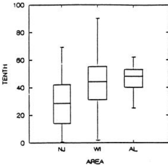
Figure 22. Tenth percentile particle sizes for stormwater inlet flows (Pitt, et al. 1997).
