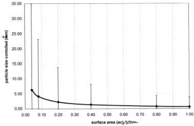
Figure 41c. Austin, TX, medium density residential area sensitivity analysis based on surface area of pond.
