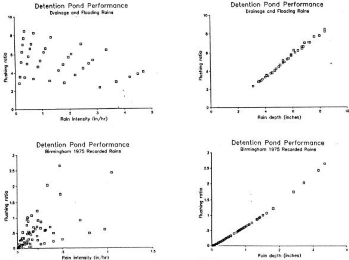
Figure 47. DETPOND modeled flushing ratios of standard pond for various rain depths and intensities.
