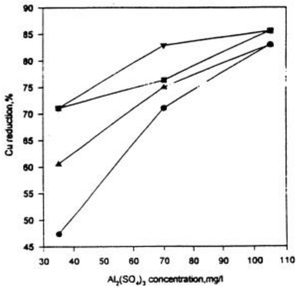
Figure 4. Copper removal using alum (Al 2 (SO 4 ) 3 )
