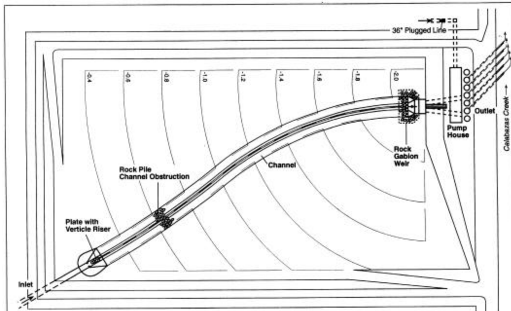
Figure 69. Sunnyvale Pump Station No. 2 dry detention pond.
