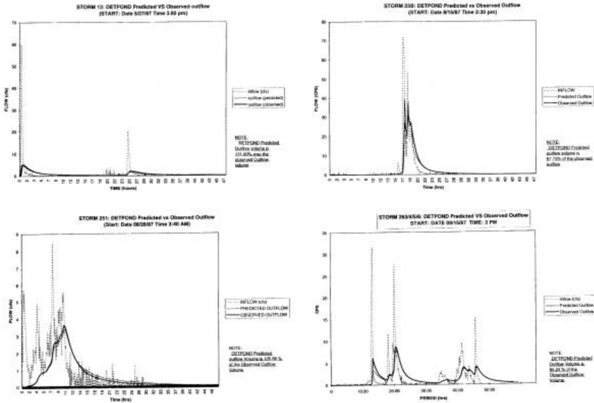
Figure 53. Predicted and observed hydrographs.
