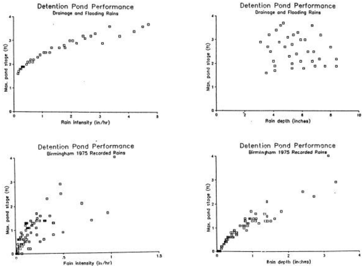
Figure 46. DETPOND modeled maximum stage of standard pond for various rain depths and intensities.
