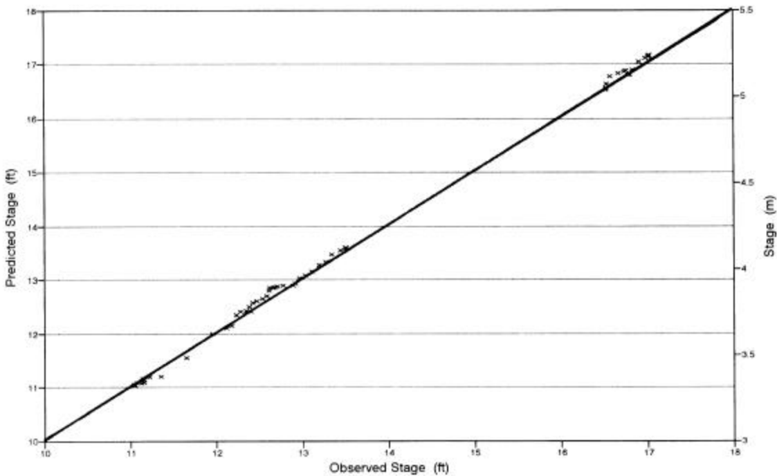
Figure 56f. Observed and predicted pond stages for Birmingham landfill pond study.
