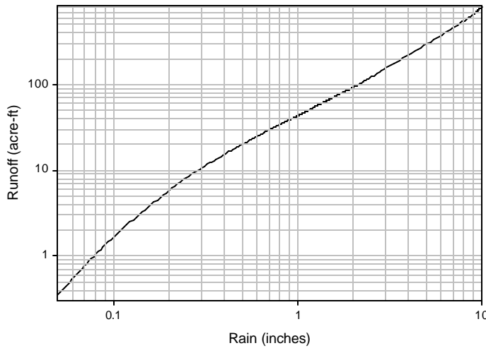
Figure 64. Rainfall-runoff relationship for airport drainage.
