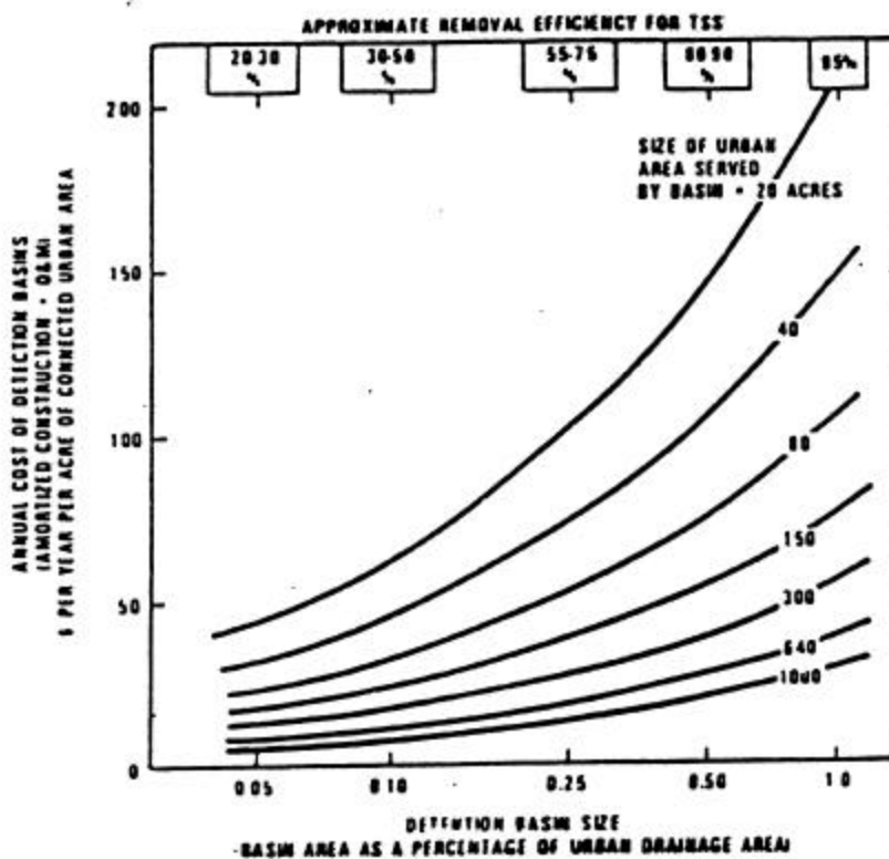
Figure 8. Detention pond costs (EPA 1983).
