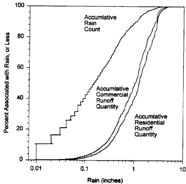
Figure 6-2. St. Louis, MO, Rain and Runoff Distributions. (1984 through 1992 rains).
