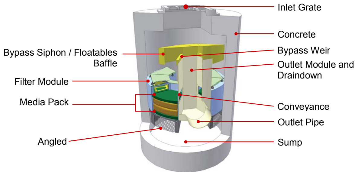
Figure 6. Up-Flo® Filter Component (Hydro International Drawing, 2010)
