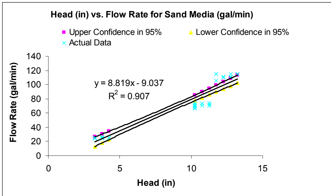
Figure 21. Flow vs. Head Graph for Sand Media (total filter surface area: 9 ft 2 )
