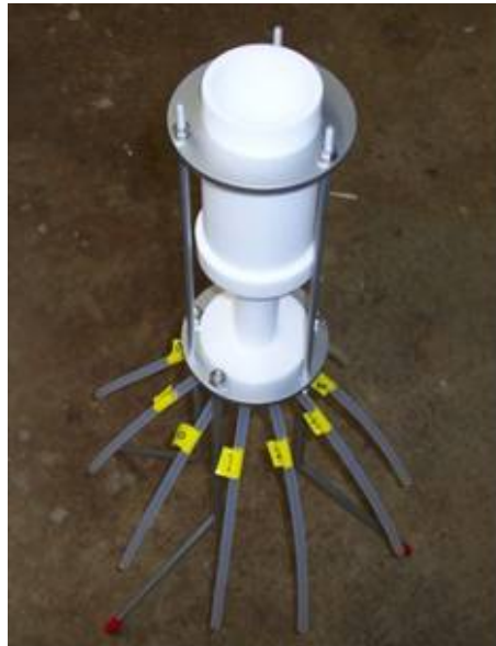
Figure 26. USGS/Dekaport Teflon™ Cone Splitter
