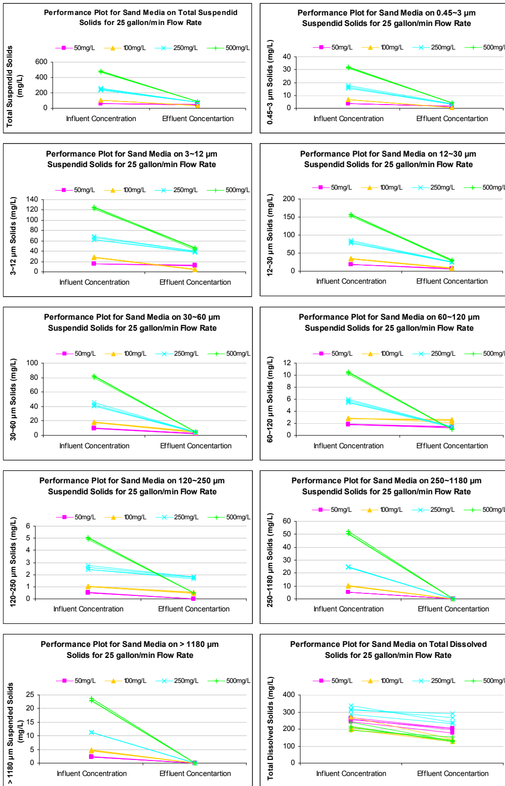
Figure 67. Sand Media 25 gpm Controlled Flow Test Results
