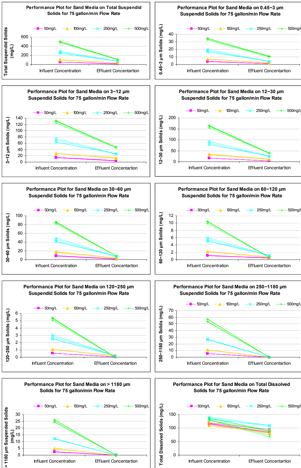
Figure 68. Sand Media 75 gpm Controlled Flow Test Results
