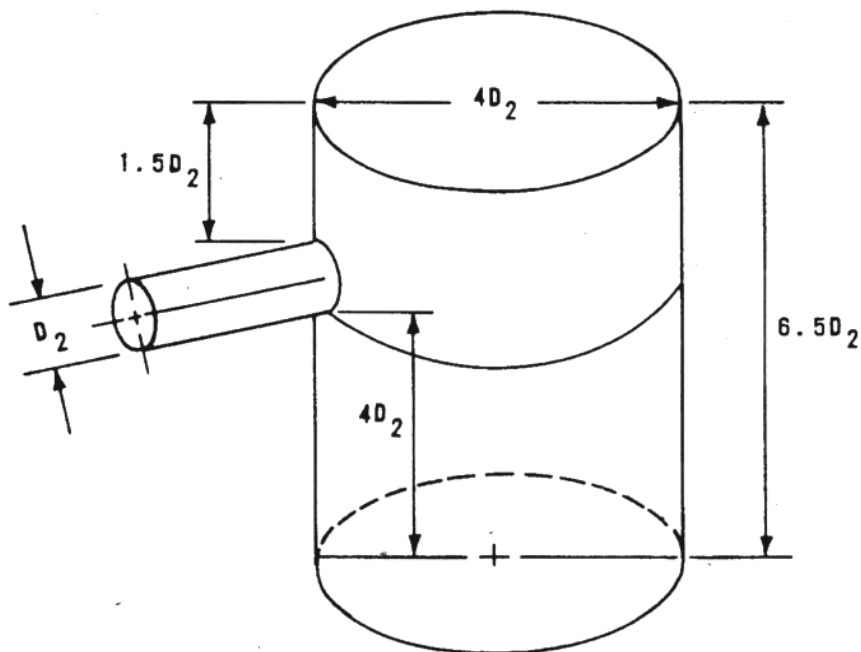
Figure 5. Recommended design (Lager et al., 1977)
