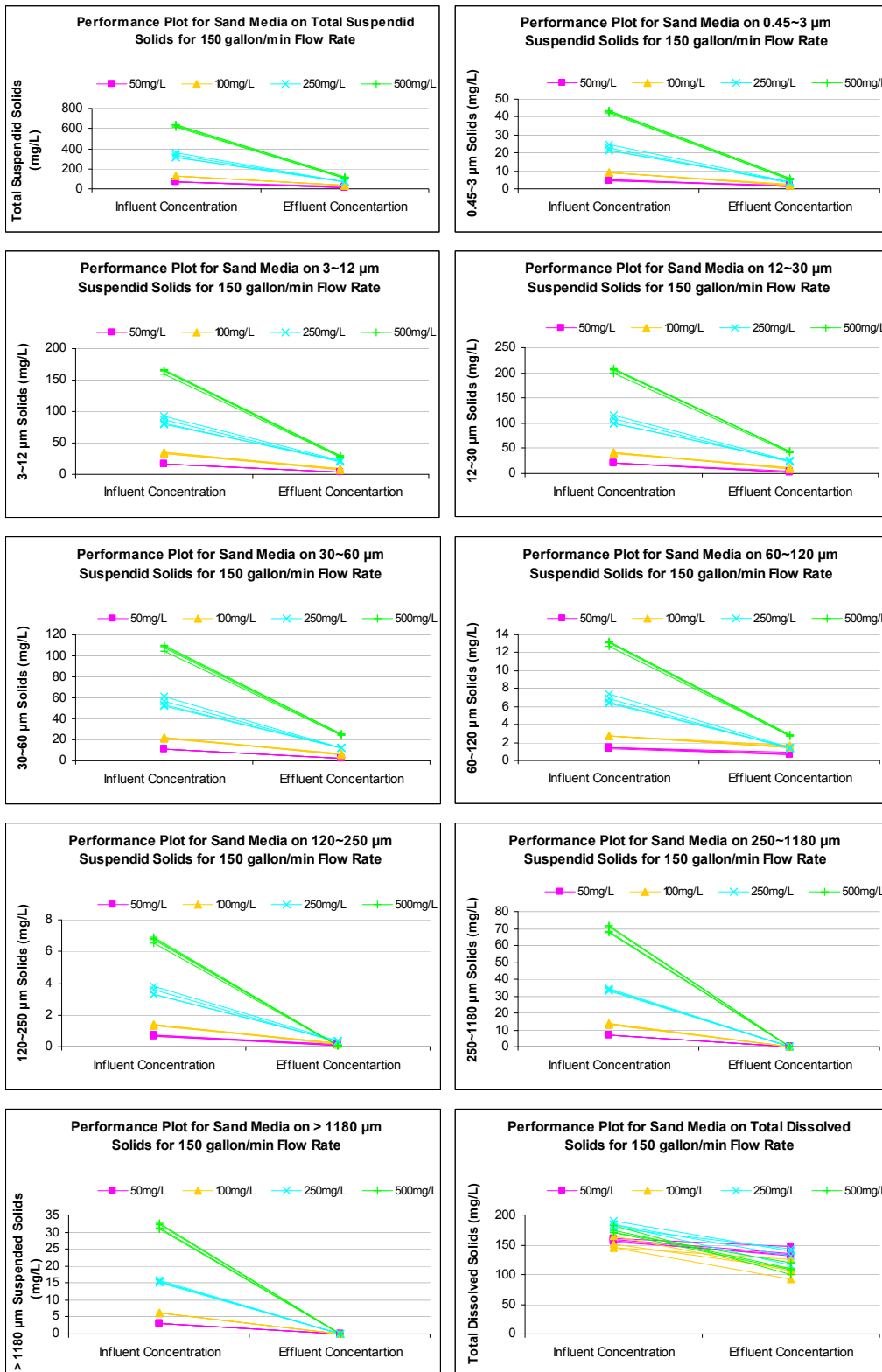
Figure 69. Sand Media 150 gpm Controlled Flow Test Results
