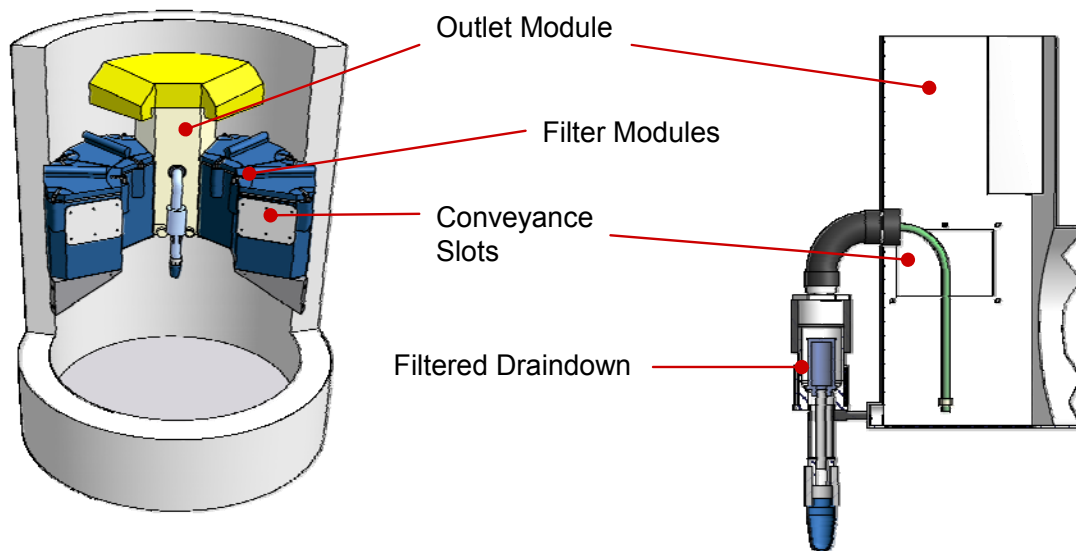
Figure 8. Outlet Module and Filtered Draindown (Hydro International Drawing, 2010)
