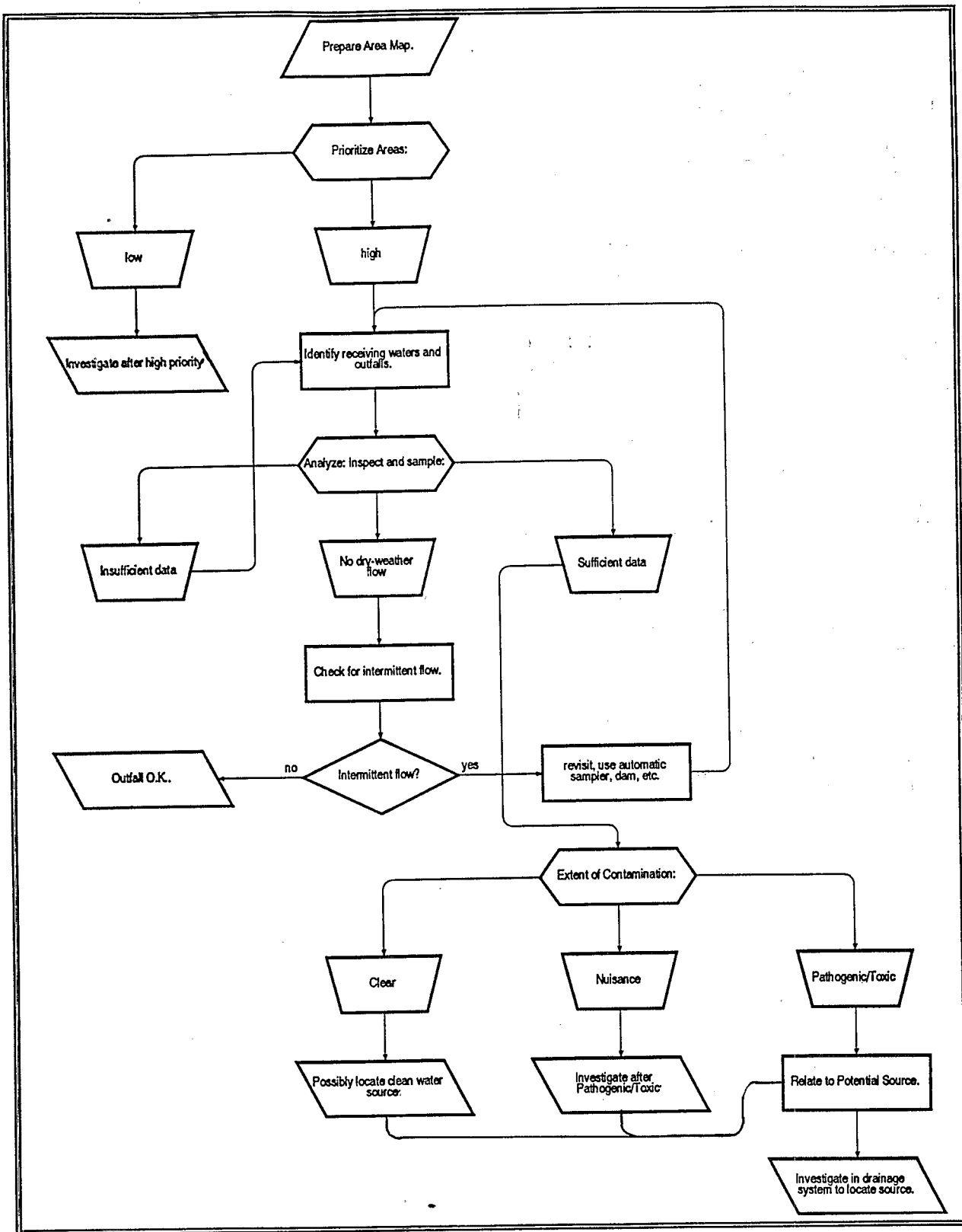
Figure 2. Flow chart for investigation procedures.
