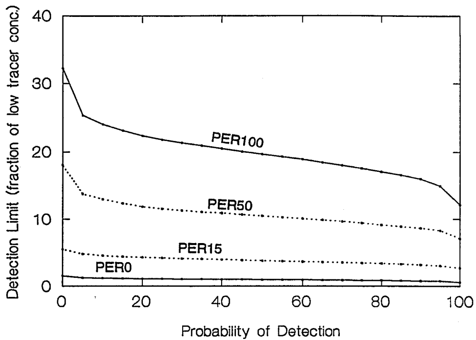
Figure 6. Required detection limits for low COV mixture components having means differing by 20 times.
